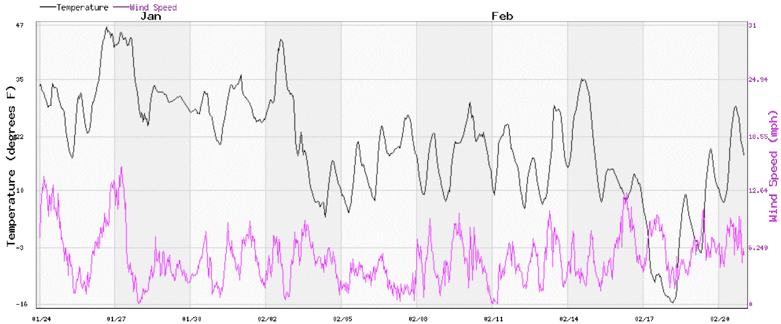
Figure 6. Temperature and Wind Speed During Period of Study
