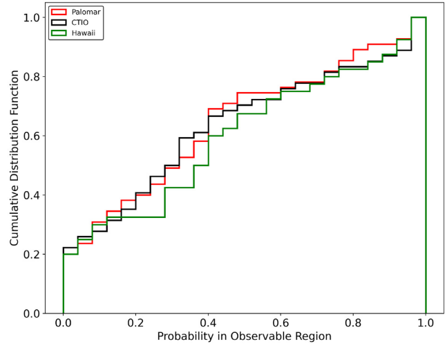
Figure 4. Probability contained within the observable region of the sky localization for all GW candidates during O3; this is shown from three different locations (Palomar ( 33.3563^\circ , -116.8648^\circ ), CTIO ( -30.1691^\circ , -70.8062^\circ ), and Hawaii ( 19.8968^\circ , 155.5828^\circ ); the LALInference sky localization was used as long as it was available for the candidate/event in question.
