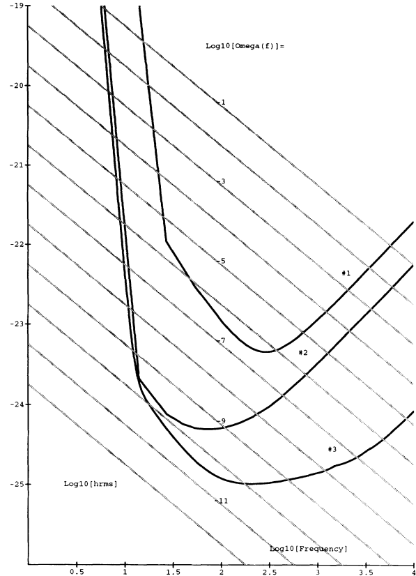
FIG. 11. Plot of sensitivity to h_{rms} and \Omega_{gw}(f) (diagonal gray lines) vs frequency for the initial recycled Fabry-Pérot (No. 1), the advanced recycled Fabry-Pérot (No. 2), and the envelope for the advanced dual-recycling Fabry-Pérot (No. 3). This assumes a 4- and a 2-km interferometer at the same site.
