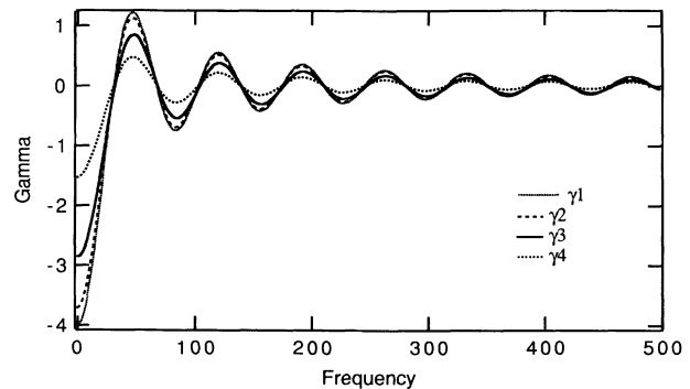
FIG. 7. Plot of \gamma vs frequency (in Hz) for the detector-1-detector-2 geometry. Detector 1 interferometer has one arm along the great circle connecting the two sites. The other interferometer has an arm along the great circle for \gamma_1 , an arm 11.25^\circ off the great circle for \gamma_2 , 22.5^\circ for \gamma_3 , and 33.75^\circ for \gamma_4 . Note that the zeros do not move.
