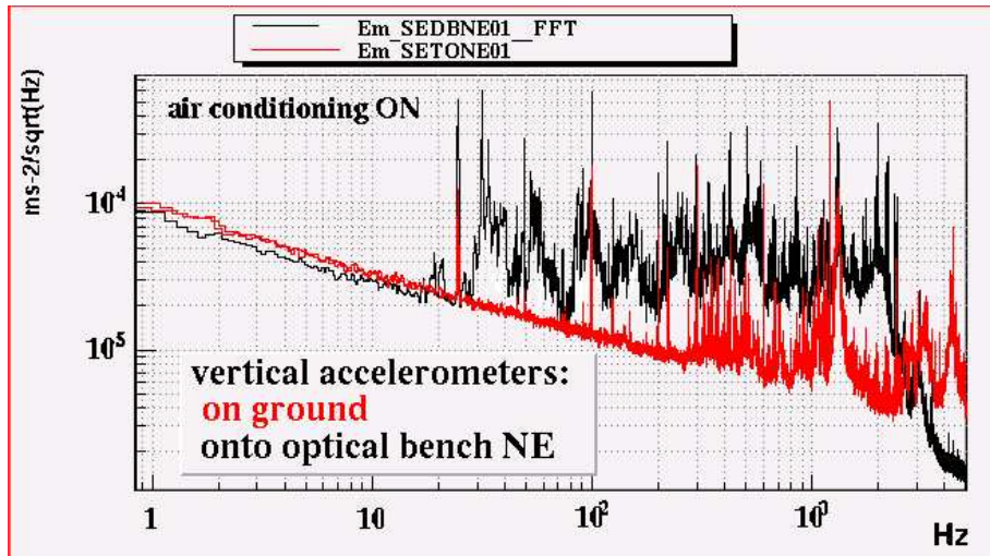
Figure 18: Seismic noise on the ground and on the NE external optical bench.
