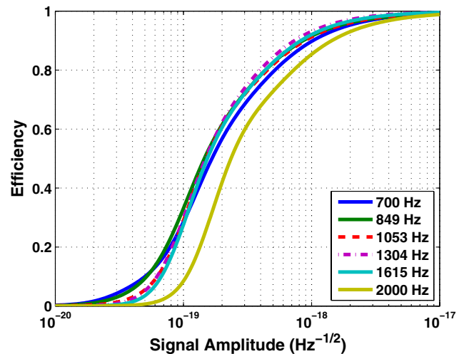
FIG. 8 (color online). Detection efficiency for the combined data set, by central frequency f_0 of the sine-Gaussian signal in Eq. (4.1). There is a statistical uncertainty at each point in these curves of approximately 2%–4% due to the finite number of simulations performed.
