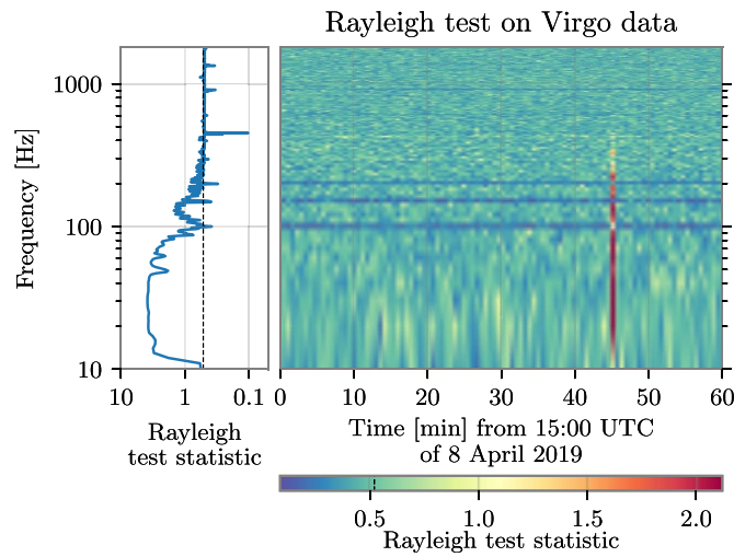
Figure 6. Example of application of the Rayleigh test, where the blue line in the left panel is the test statistic estimated over the entire hour of data, while the color map corresponds to ASD estimates over 10 s of data. The vertical dashed black line on the left plot indicates the 0.52 limit value. See text for details.
